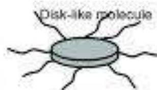
Nematic phase
